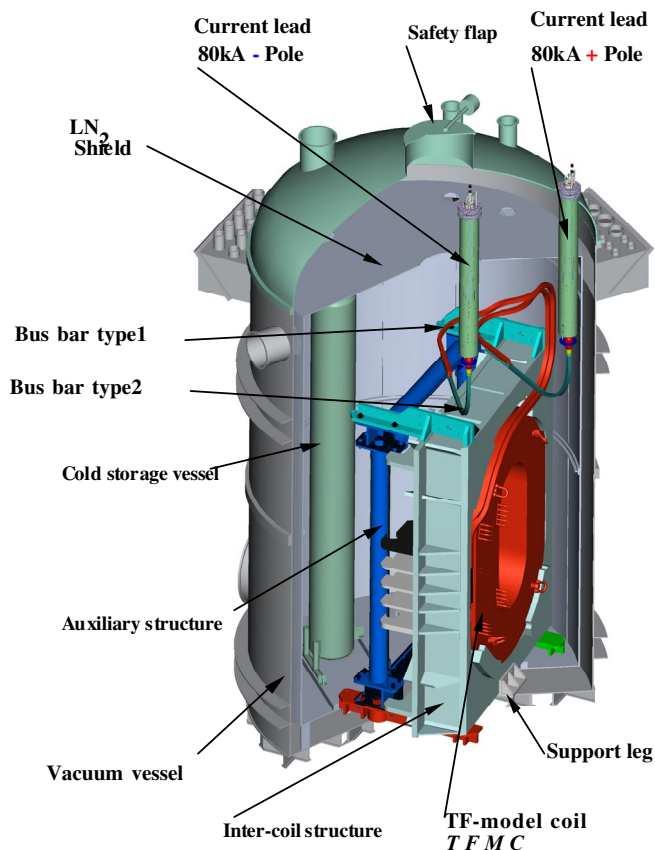
Fig. 3: The test rig to test the TFMC alone in the TOSKA facility of the Forschungszentrum Karlsruhe
